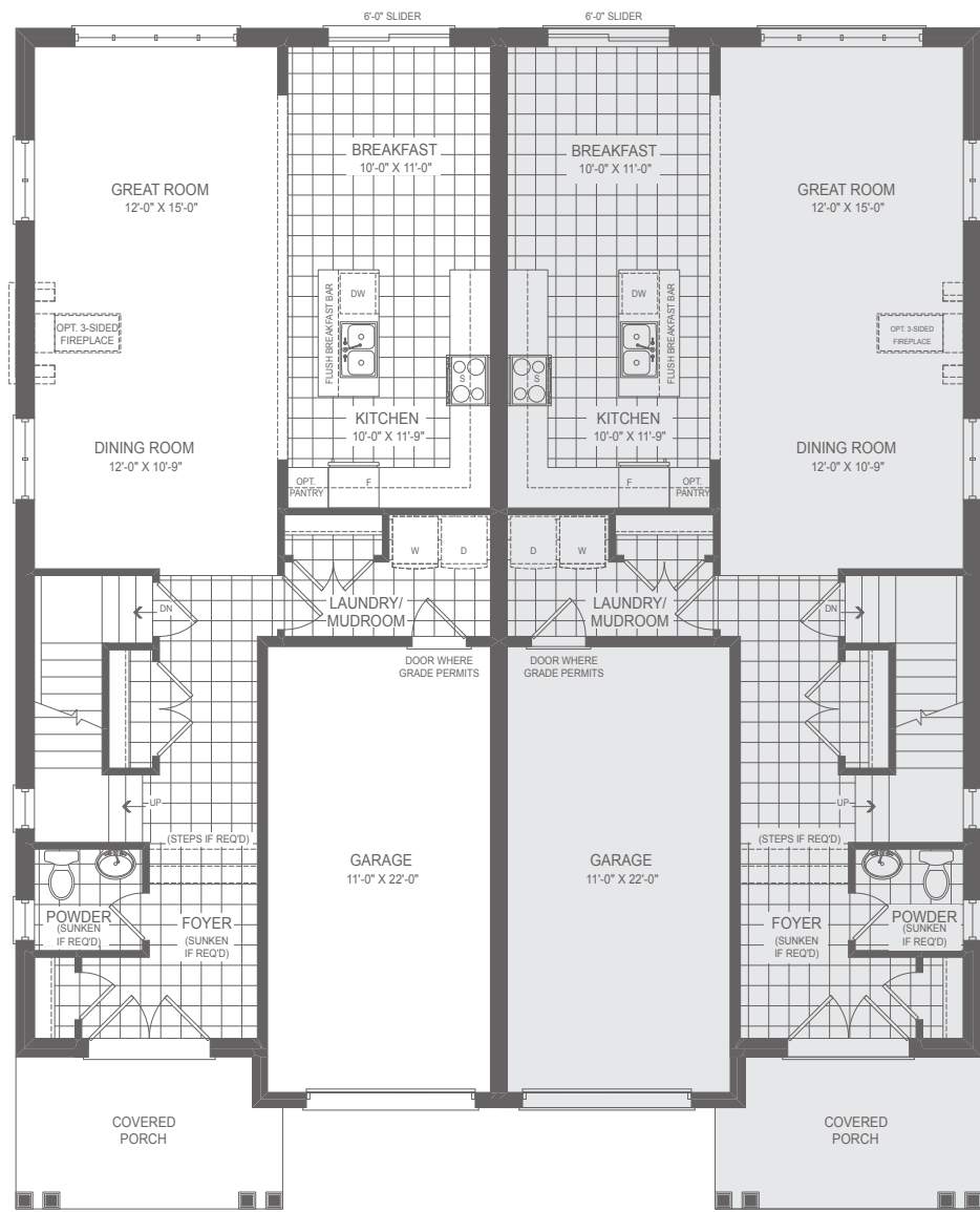
MAIN FLOOR [L] ELEVATION A
