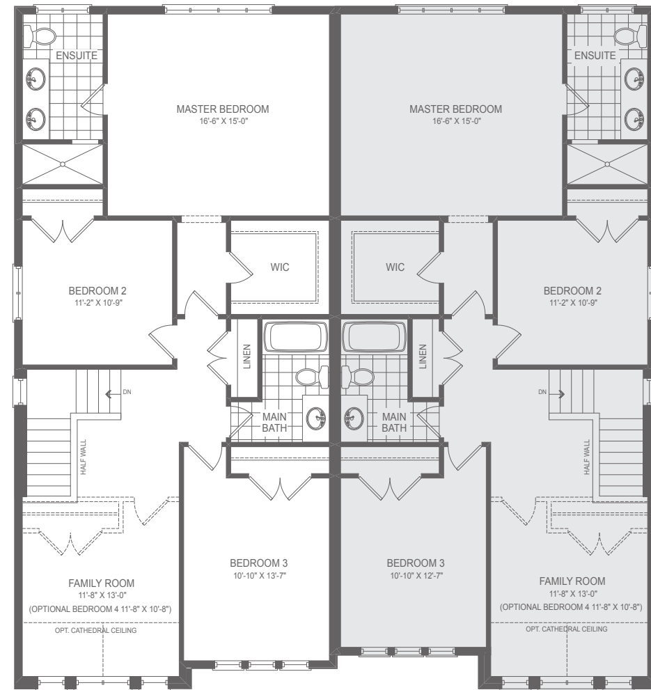
SECOND FLOOR [L] ELEVATION A
