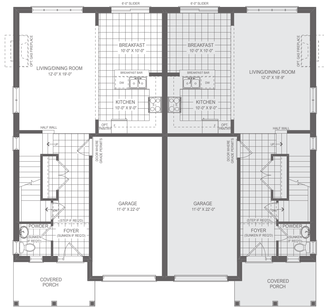
MAIN FLOOR [L] ELEVATION A
